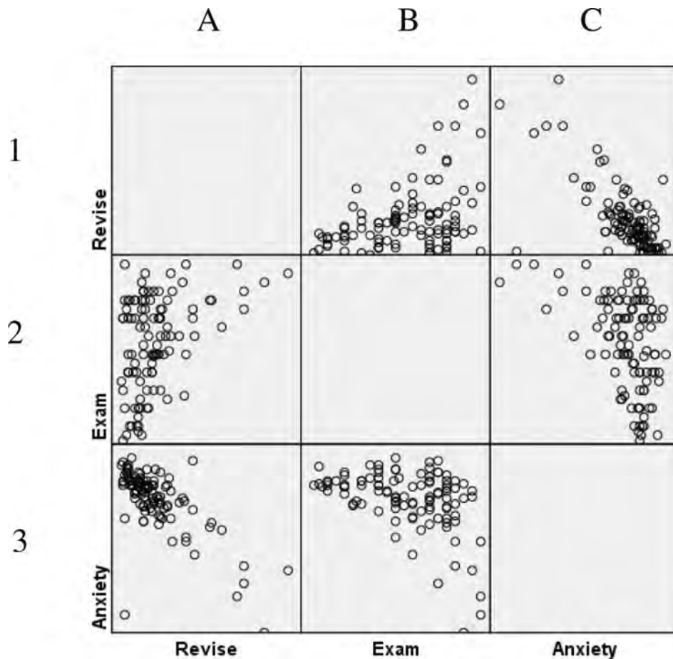
FIGURE 4.39 Matrix scatterplot of exam performance, exam anxiety and revision time. Grid references have been added for clarity
