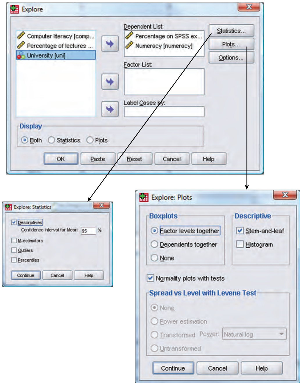
FIGURE 5.9 Dialog boxes for the explore command
