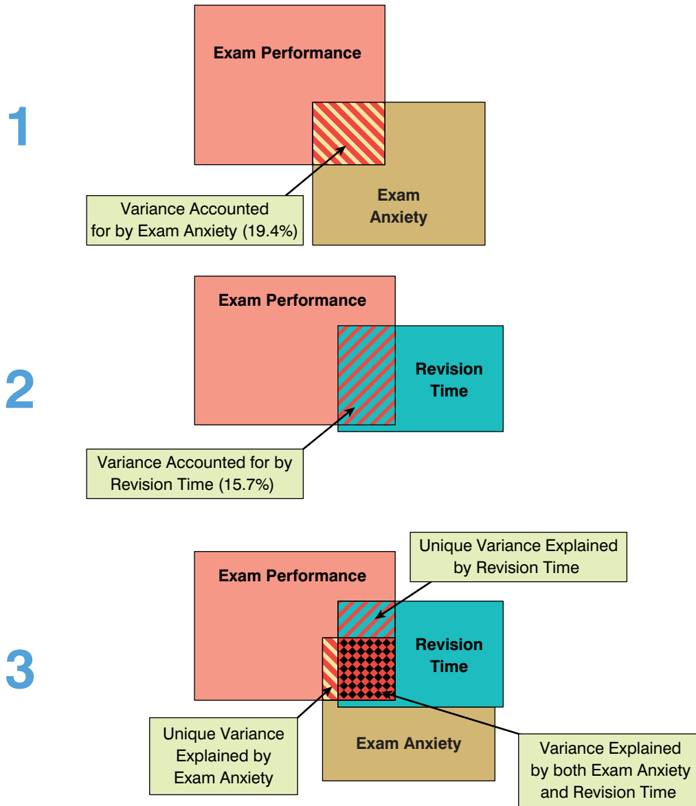
FIGURE 6.9 Diagram showing the principle of partial correlation
