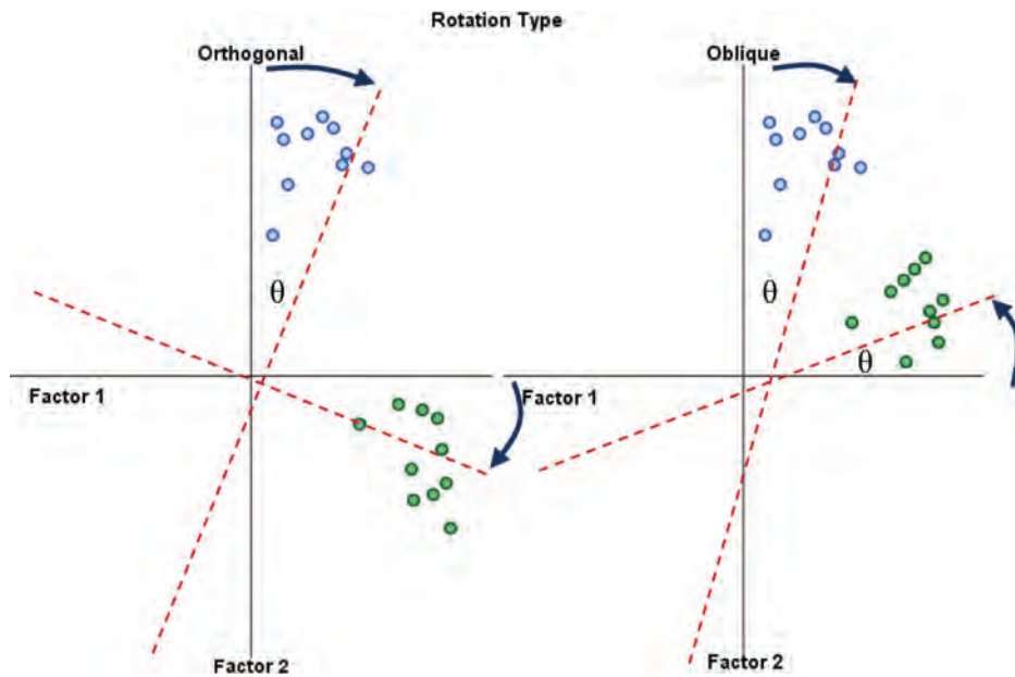
FIGURE 17.4 Schematic representations of factor rotation. The left graph displays orthogonal rotation whereas the right graph displays oblique rotation (see text for more details). \theta is the angle through which the axes are rotated
