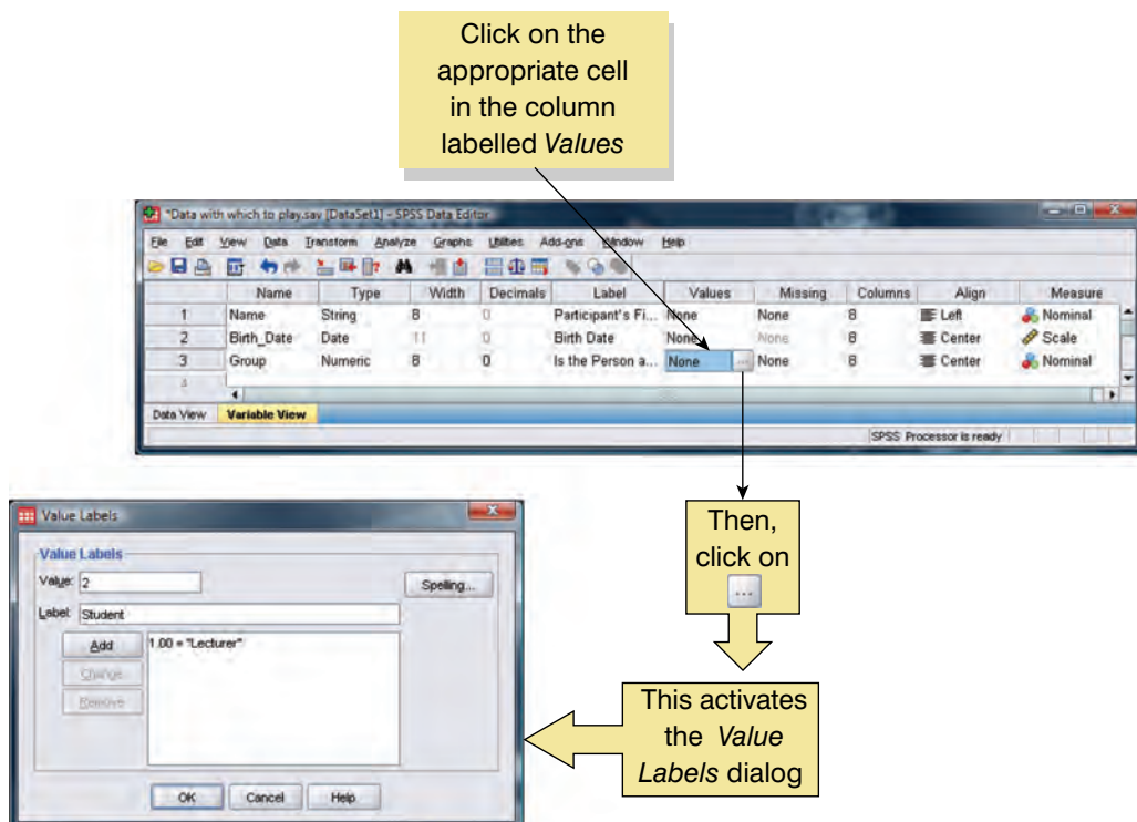
FIGURE 3.7 Defining coding variables and their values in SPSS
