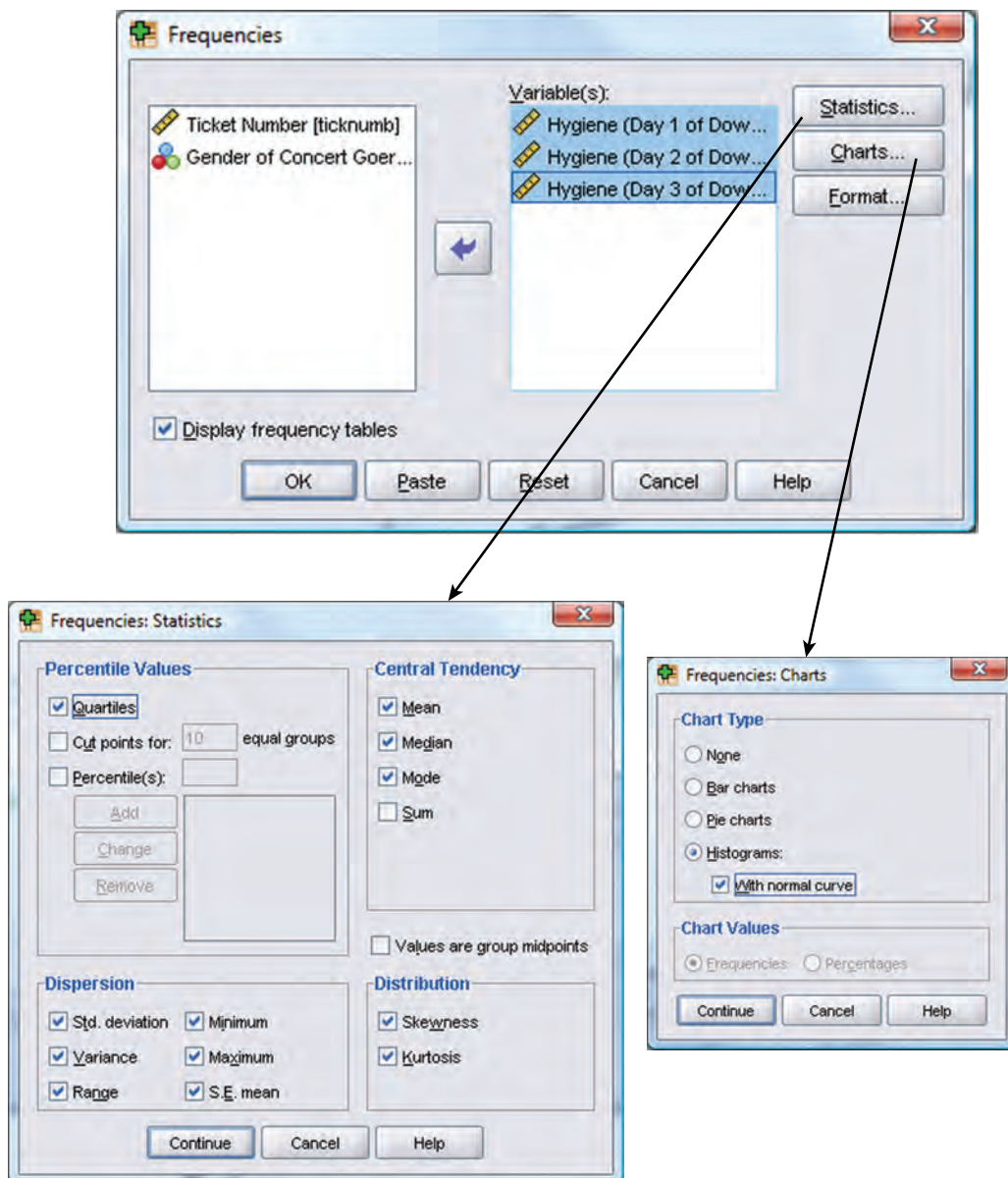
FIGURE 5.4 Dialog boxes for the frequencies command
