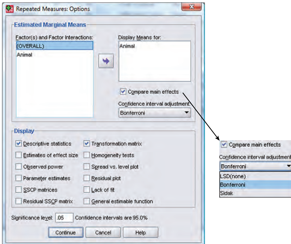
FIGURE 13.6 The options dialog box
